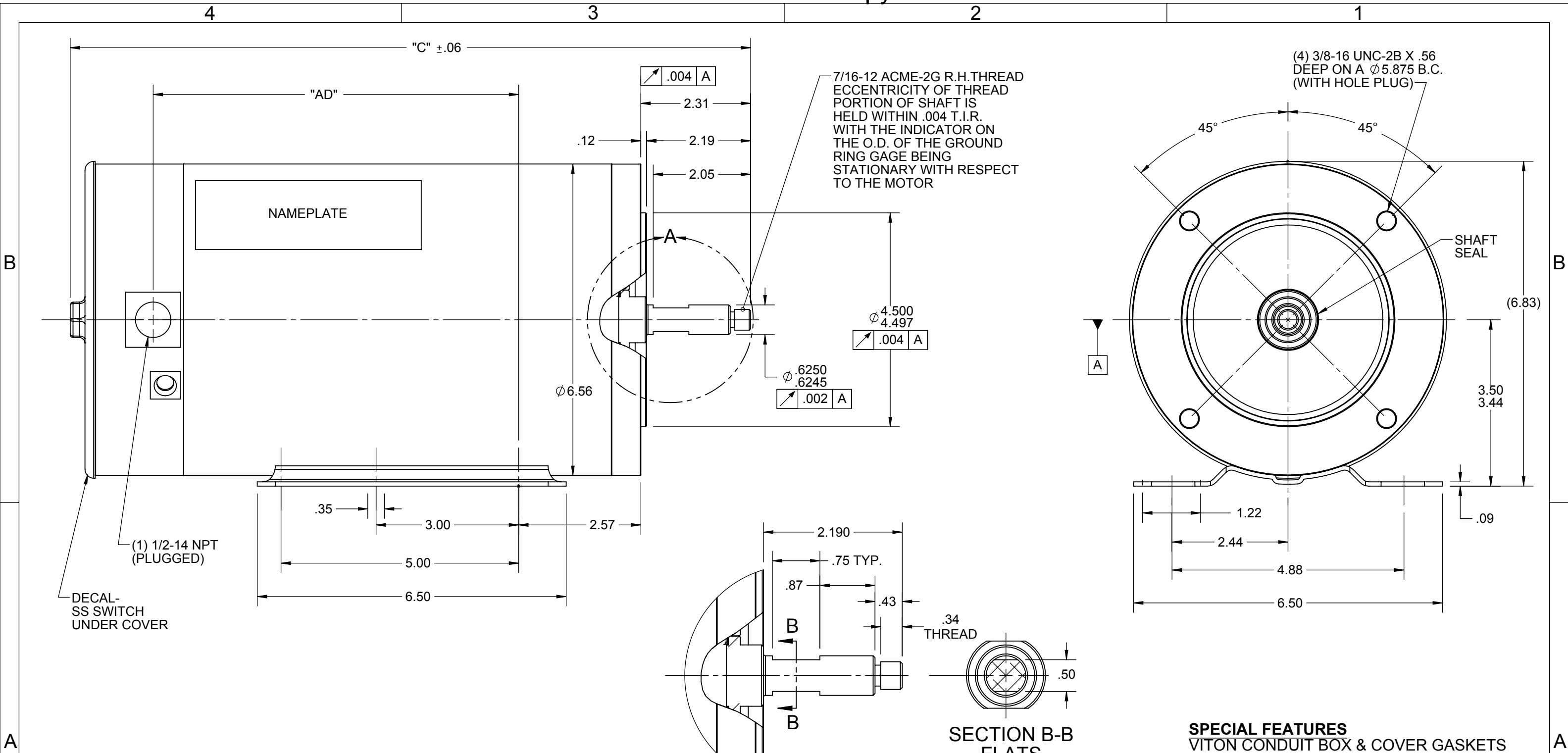
DETAIL A SHAFT DETAIL
