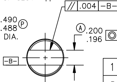
VIEW X-X ENLARGED VIEW OF SLOT
