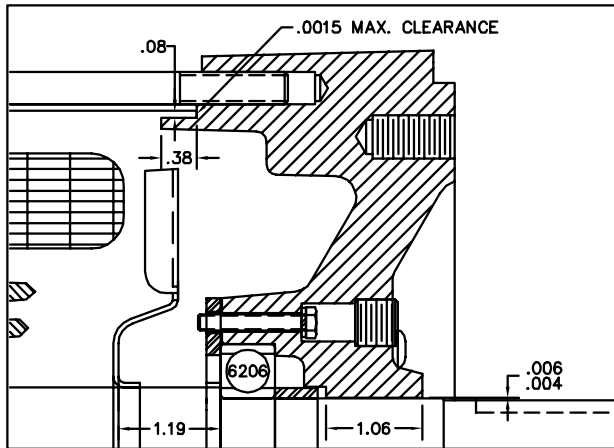
PULLEY END DETAIL
