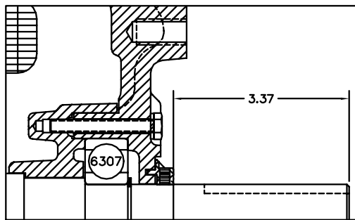
PULLEY END DETAIL
