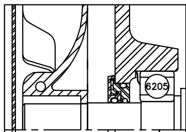
FRONT END DETAIL
