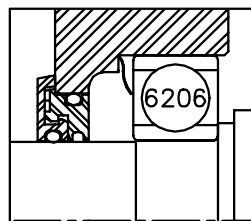
FRONT END DETAIL
