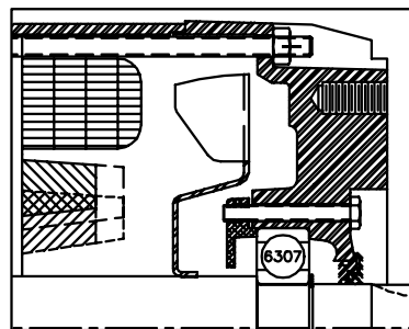
PULLEY END DETAIL
