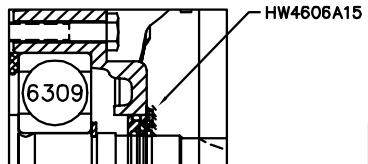
PULLEY END DETAIL
