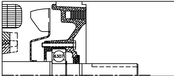
PULLEY END SECTION
