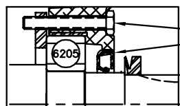
PULLEY END DETAIL
