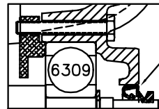
PULLEY END DETAIL
