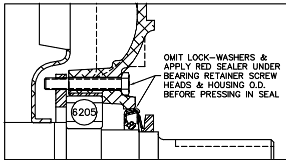
PULLEY END DETAIL
