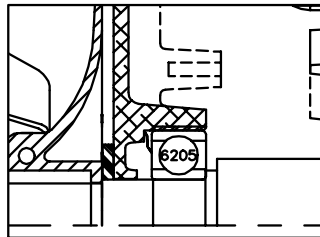
FRONT END SLINGER DETAIL
