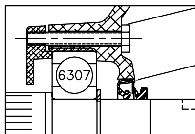
PULLEY END DETAIL
