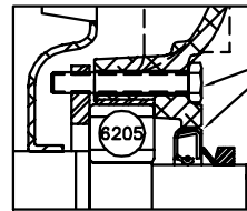
PULLEY END DETAIL
