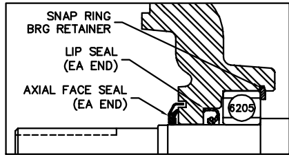
PULLEY END DETAIL
