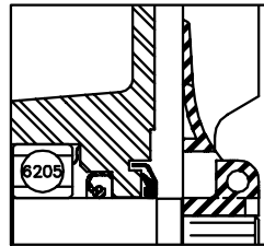
FRONT END DETAIL
