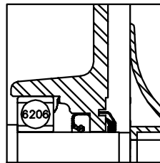
FRONT END DETAIL
