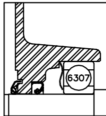
FRONT END DETAIL
