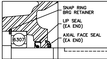
PULLEY END DETAIL
