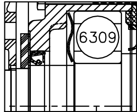
FR LIP SEAL DETAIL
