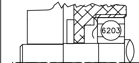
FRONT END DETAIL
