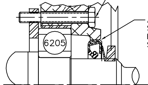
PULLEY END DETAIL
