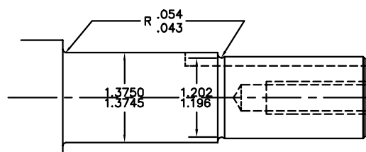
UNDERCUT DETAIL SCALE = .75
