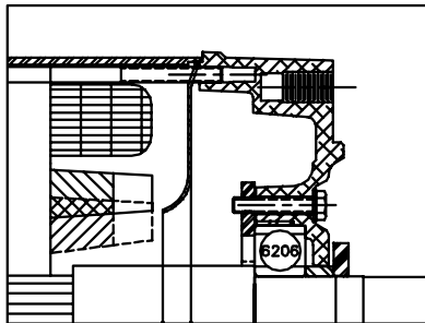
PULLEY END DETAIL
