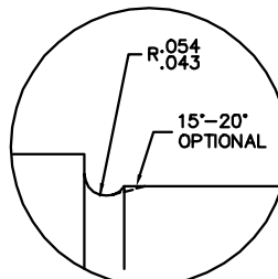
UNDERCUT DETAIL
