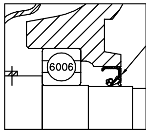
PULLEY END
