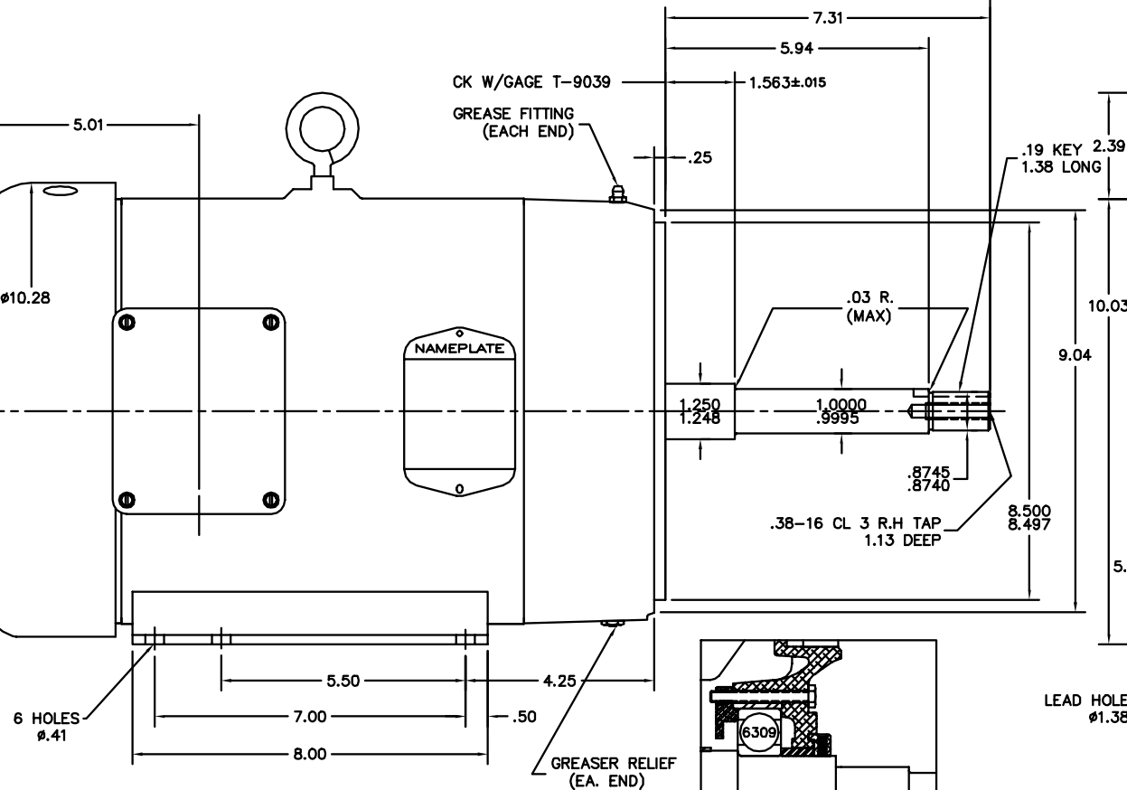
PULLEY END DETAIL
