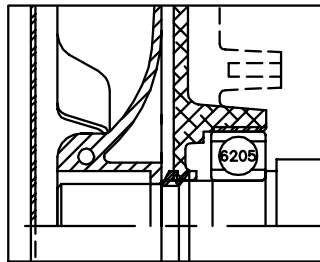
FRONT END SLINGER DETAIL
