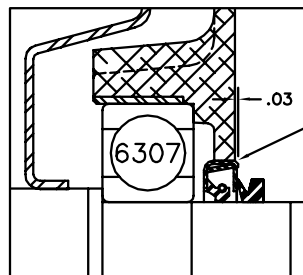
PULLEY END DETAIL
