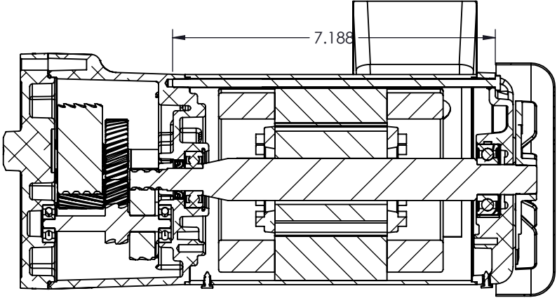
SECTION R-R
