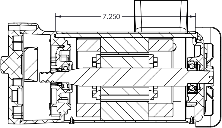
SECTION R-R
