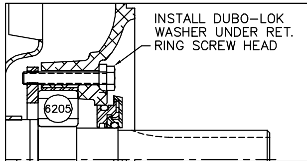
PULLEY END DETAIL
