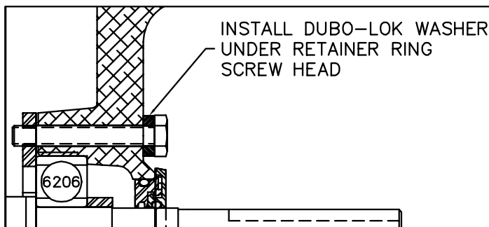
PULLEY END DETAIL
