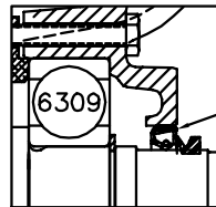
PULLEY END DETAIL
