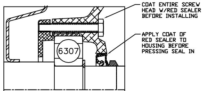
PULLEY END DETAIL
