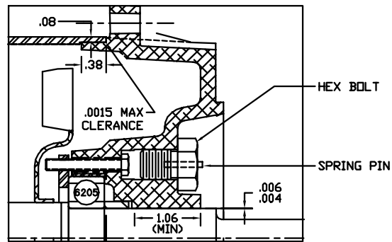
PULLEY END DETAIL
