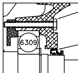
SEAL DETAIL
