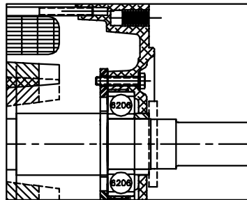
PULLEY END DETAIL
