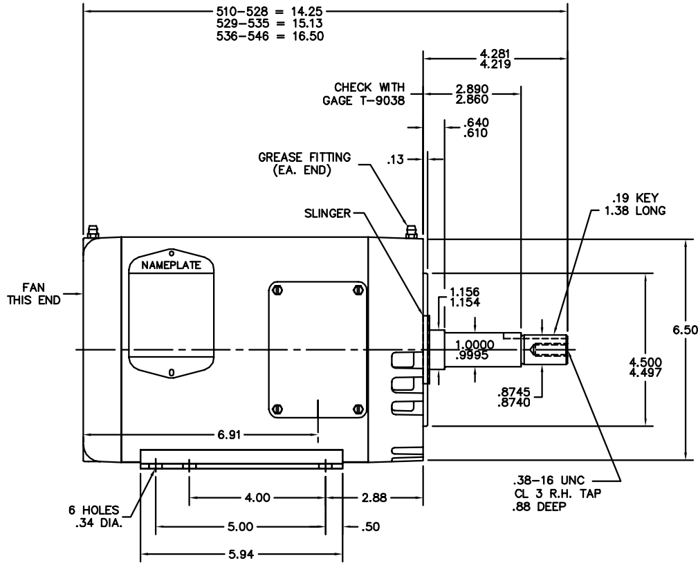
PULLEY END DETAIL
