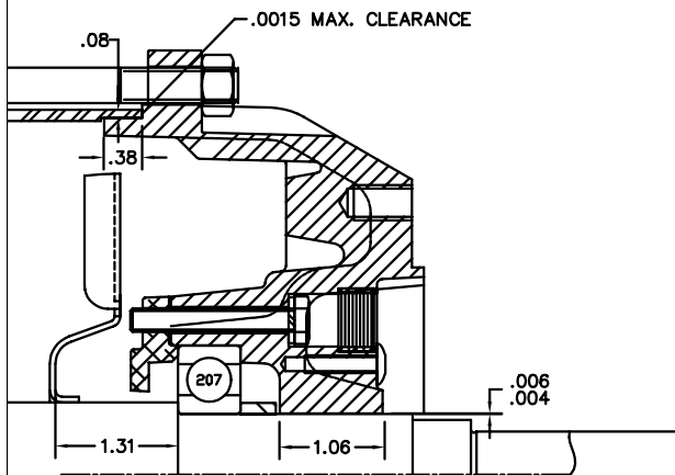
PULLEY END DETAIL
