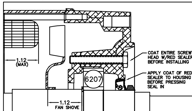
PULLEY END DETAIL
