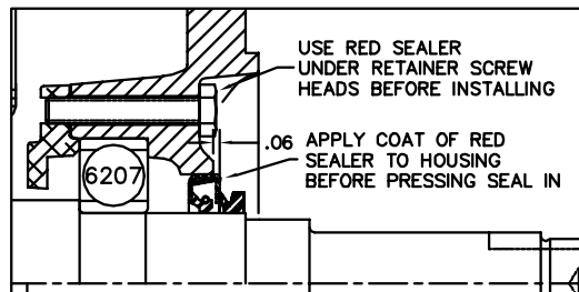
PULLEY END SEAL AND SLINGER DETAIL
