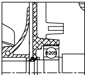
FRONT END SLINGER DETAIL
