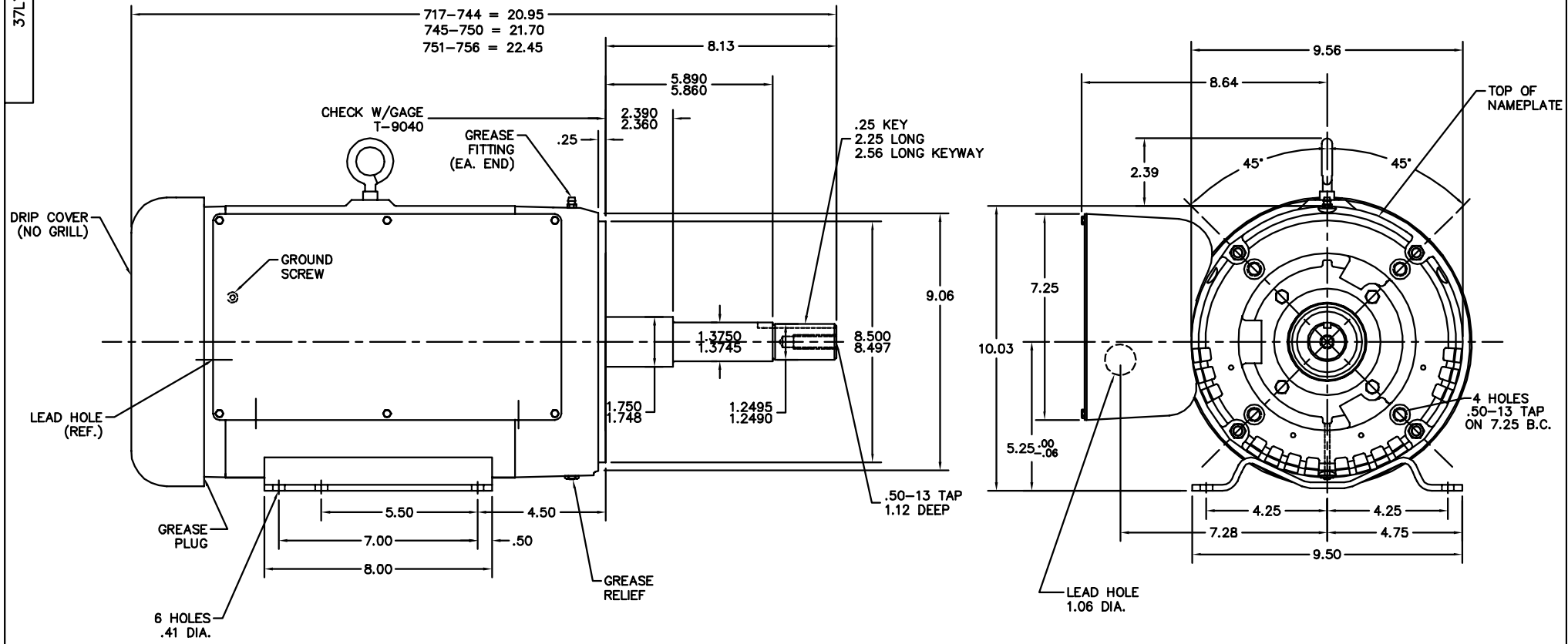
PULLEY END DETAIL
