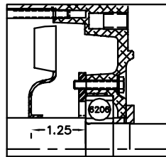
PULLEY END DETAIL
