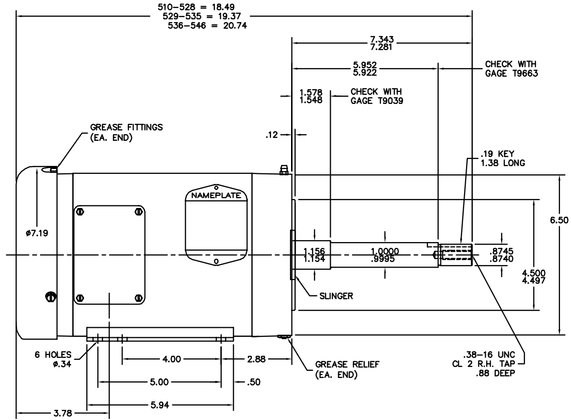
PULLEY END DETAIL
