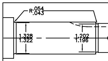
UNDERCUT DETAIL SCALE = .625
