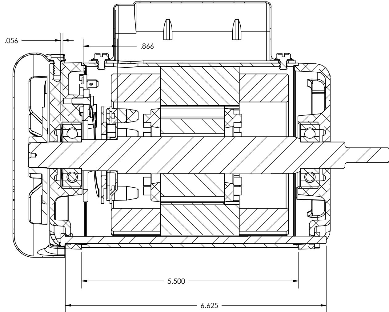
SECTION B-B
