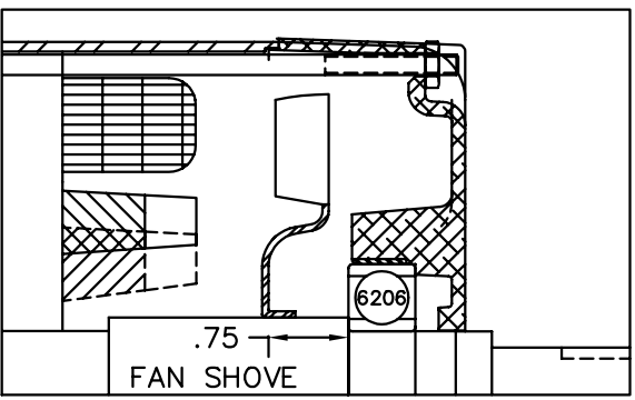
PULLEY END SECTION
