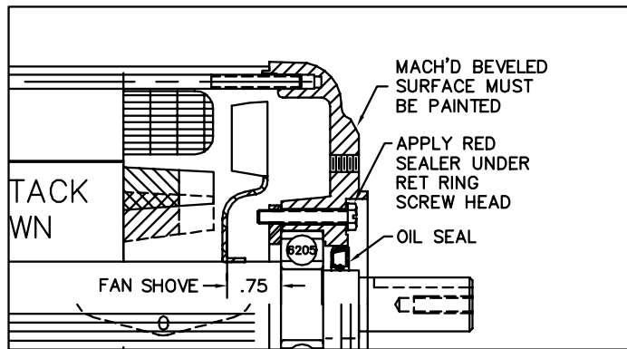
PULLEY END SECTION
