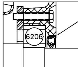
PULLEY END DETAIL
