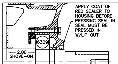
PULLEY END SECTION
