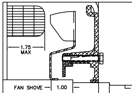
PULLEY END DETAIL
