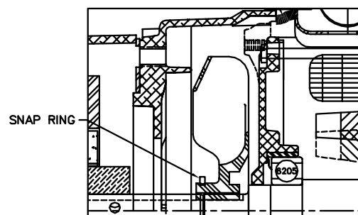
FRONT END DETAIL
