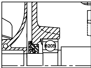
FRONT END SLINGER DETAIL
