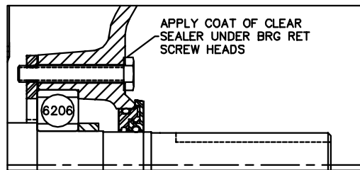
PULLEY END SEAL AND SLINGER DETAIL
