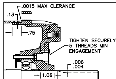
PULLEY END DETAIL
